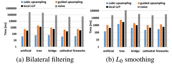
Figure 6: Computational time for each image and method.
