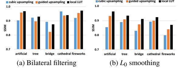
Figure 5: Approximation accuracy of SSIM for each image and method.
