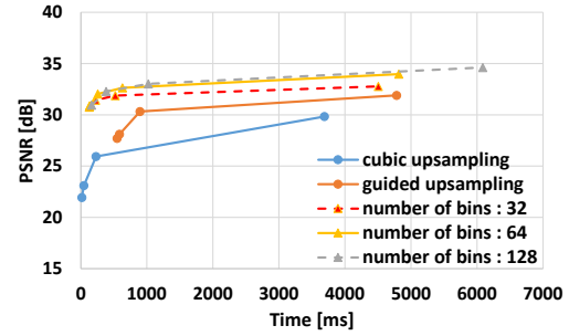
Figure 9: Resizing and changing the number of bins performance in PSNR w.r.t. computational time (bilateral filter). Local LUT samples 32, 64, and 128 bins, respectively.
