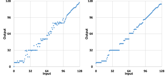
(b) Winner-takes-all
