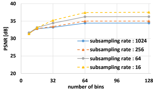
Figure 8: L_0 smoothing result: PSNR w.r.t. the number of bins with changing resizing ratio.
