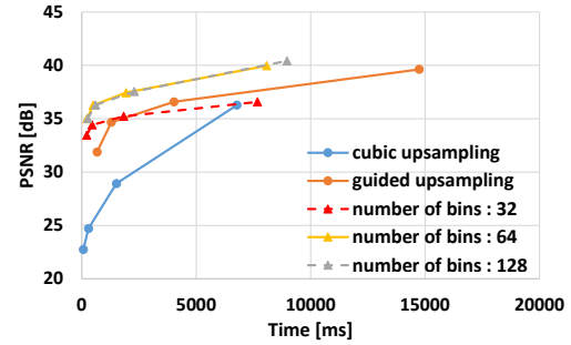
Figure 10: Resizing and changing the number of bins performance in PSNR w.r.t. computational time ( L_0 smoothing). Local LUT samples 32, 64, and 128 bins, respectively.
