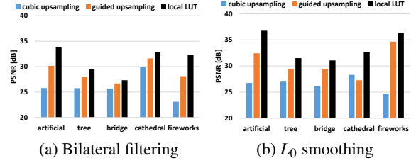
Figure 4: Approximation accuracy of PSNR for each image and method.
