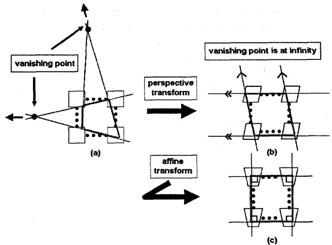
Fig. 5. Process flowchart of method A: Fig.(a) shows trajectory of characteristic point and vanishing point in input image. Fig.(b) shows trajectory of characteristic point after using perspective transformation. Fig.(c) shows trajectory of characteristic point after using affine transformation and ideal images.
