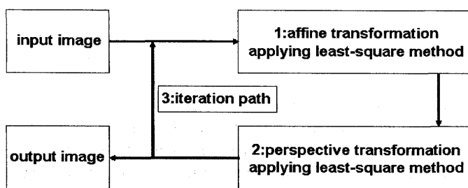
Fig. 6. Process flowchart of method B
