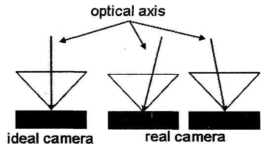
Fig. 3. individual difference
